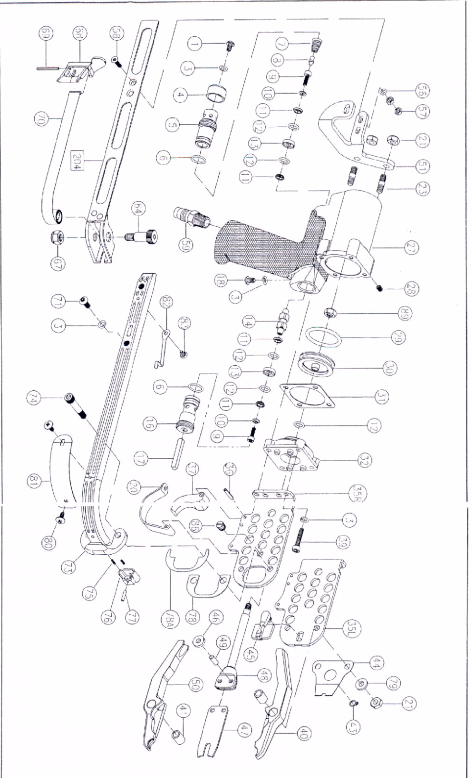
NO.202 Assembly 47,48,49
