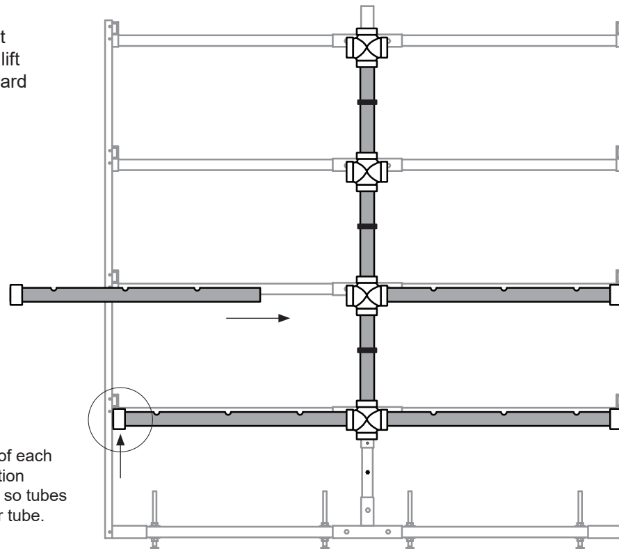
Drain manifold complete with all horizontal tubes installed.
