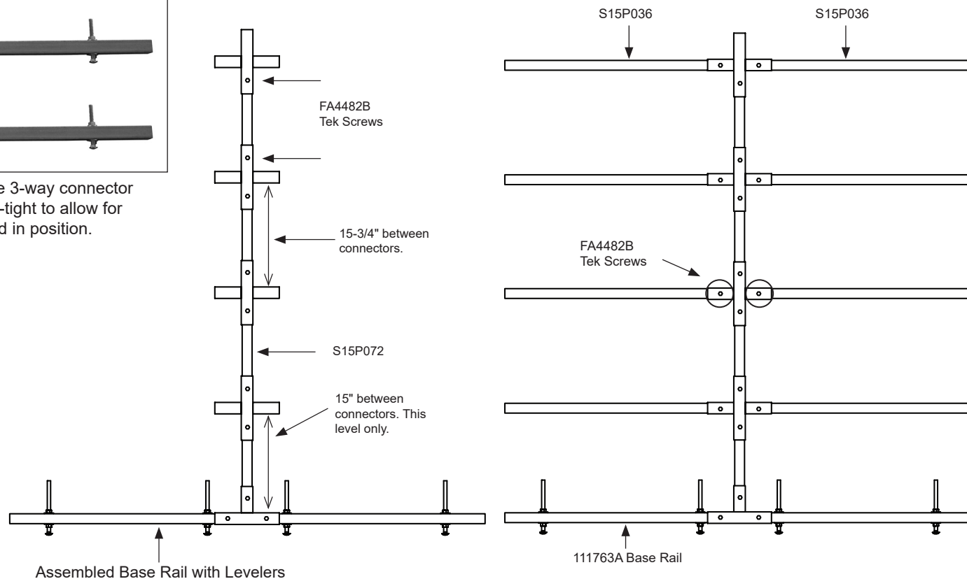
FIGURE 3: Center the connector on the base rail and secure using two (2) FA4482B Tek screws.
