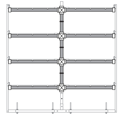
Drain manifold complete with all horizontal tubes installed.
