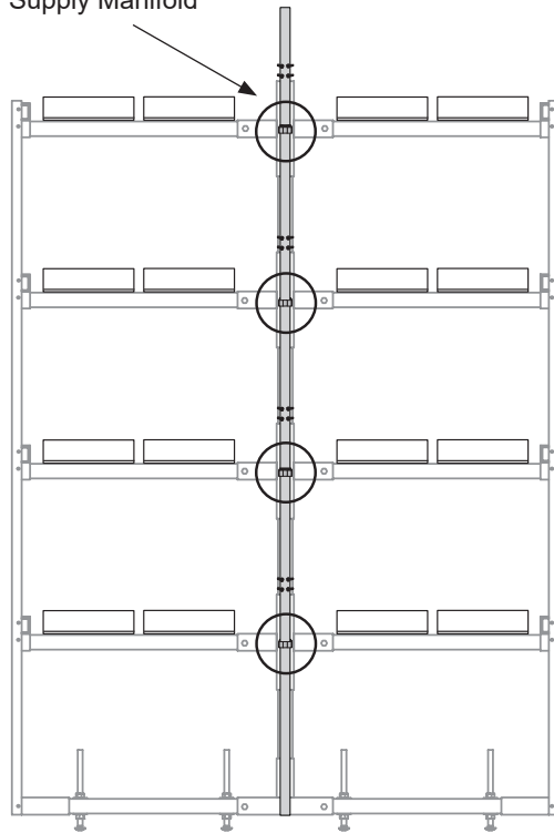
1. Attach hangers and manifold to frame.
