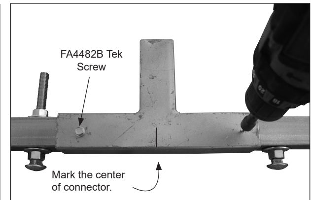
FIGURE 3: Center the connector on the base rail and secure using two (2) FA4482B Tek screws.
