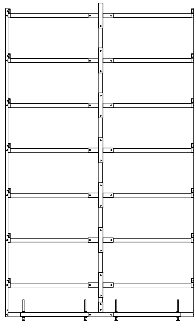
Diagram above shows the end frame for your 111628E FodderPro 2.0 Full Feed System — Expanded.
