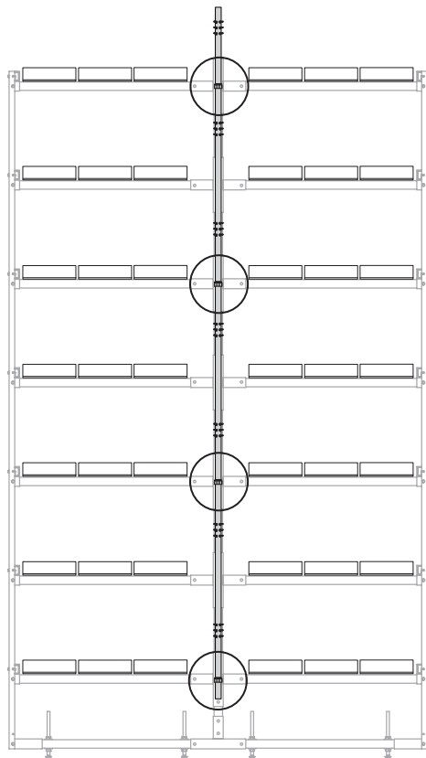
1. Attach hangers and manifold to frame.
