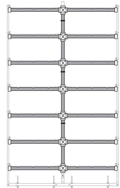
Drain manifold complete with all horizontal tubes installed.
