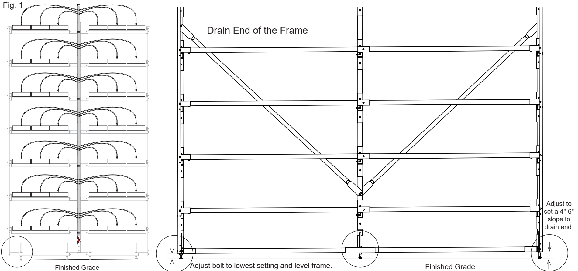
Photo shows the levelers as attached to the base rail of the end frame. Actual bolt may differ.
