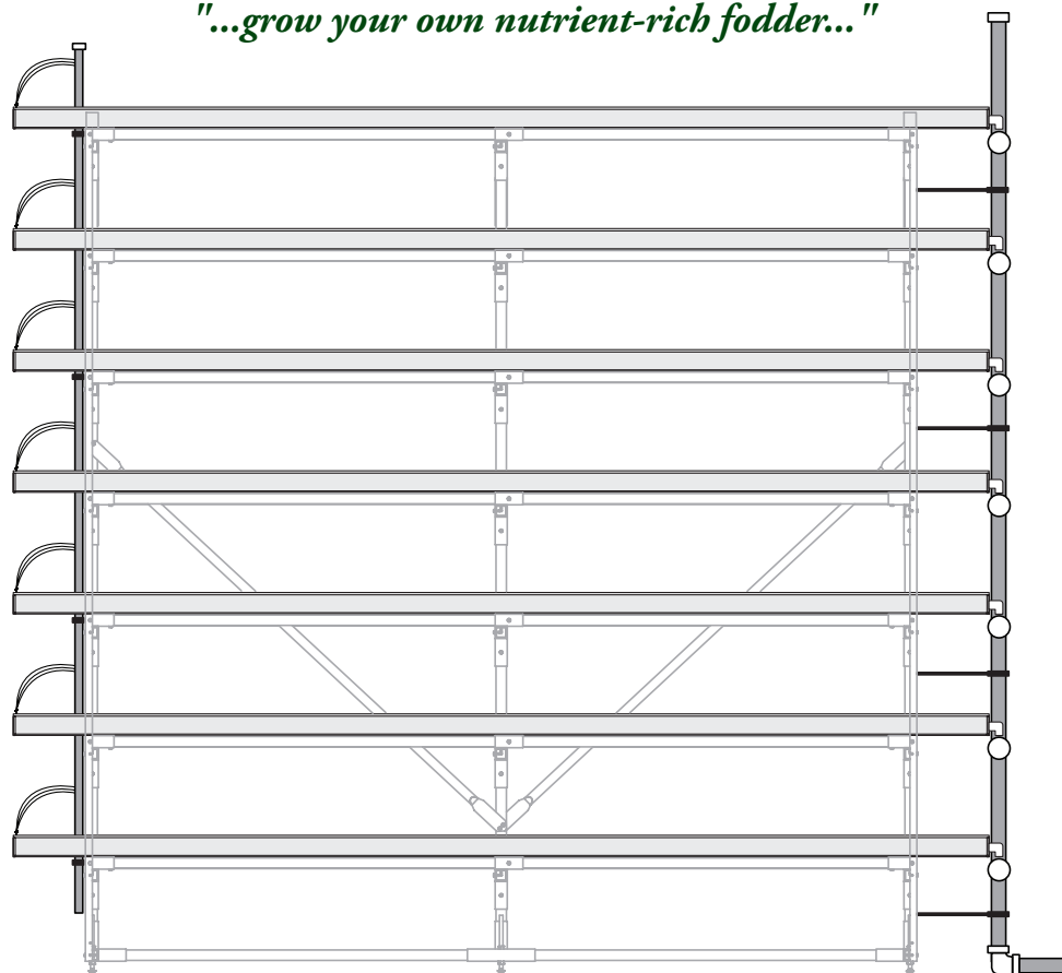
Side View with Channels and Manifolds Installed
