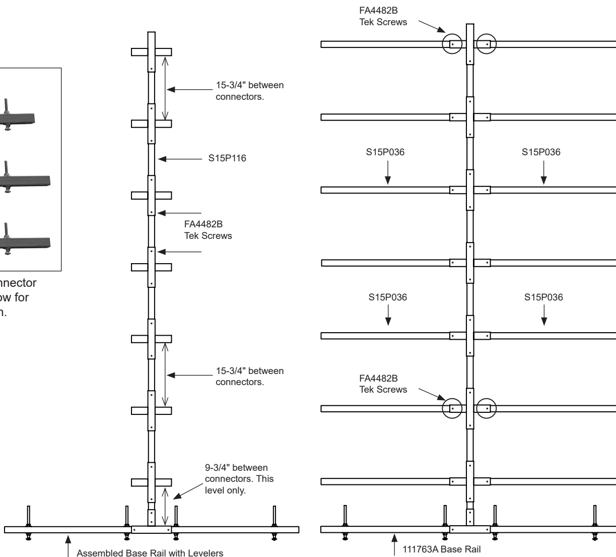
FIGURE 3: Center the connector on the base rail and secure using two (2) FA4482B Tek screws.
