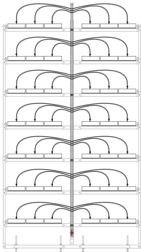
End View Shows Supply Manifold and Channels
