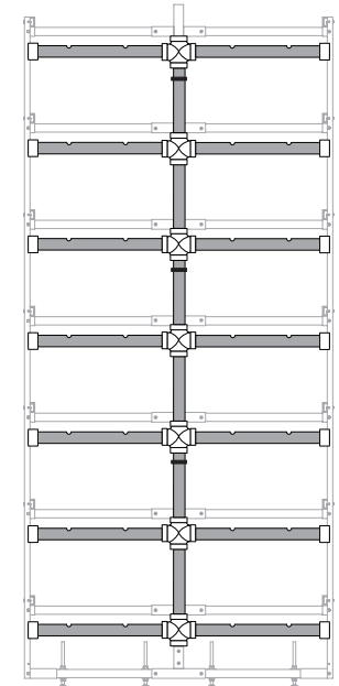
Drain manifold complete with all horizontal tubes installed.
