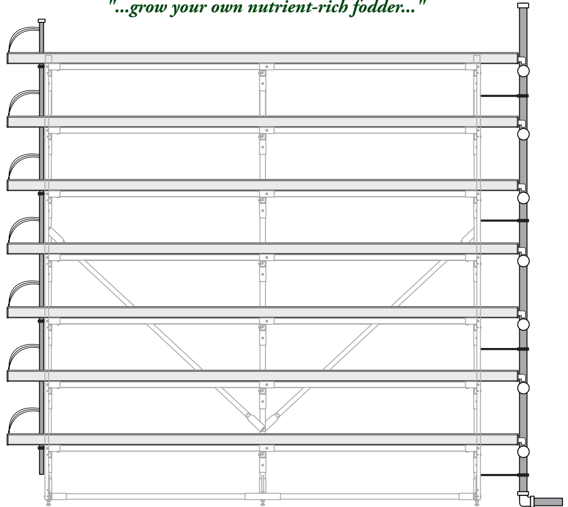
Side View with Channels and Manifolds Installed
