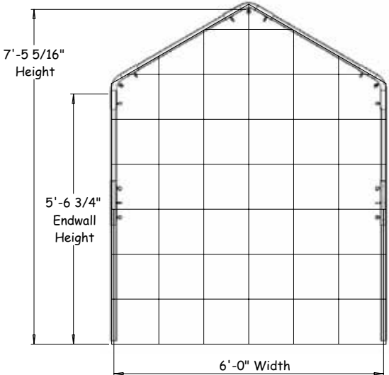
FRONT Grid Represents 12" Squares
