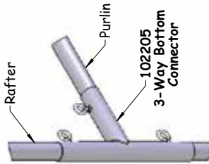
View 4 End Rafter- Bottom Purlin Connection
