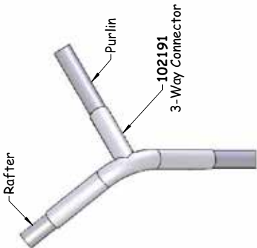
View 1 End Rafter-Purlin Connection
